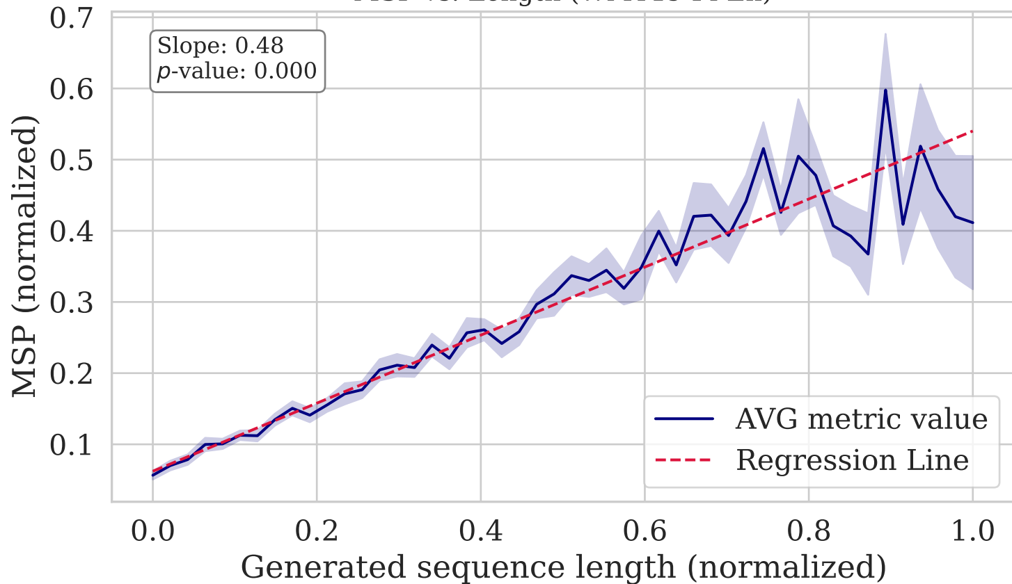
MSP vs. Length (WMT19 Fi-En)
