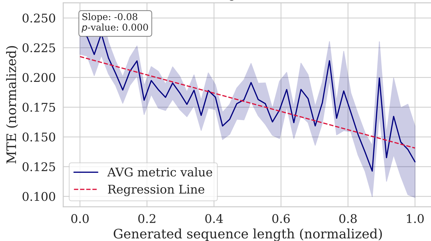
MTE vs. Length (WMT19 Fi-En)
