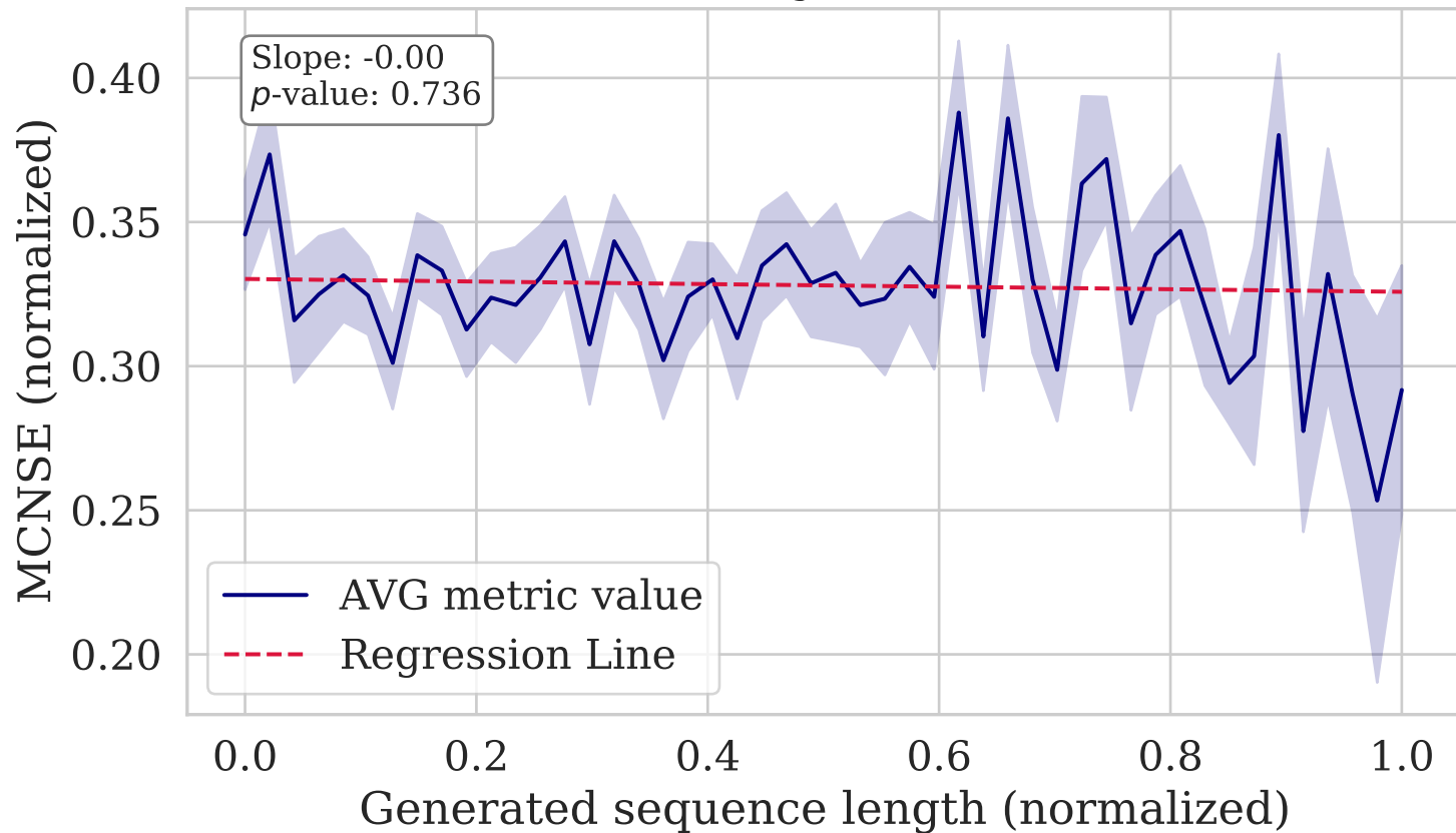
MCNSE vs. Length (WMT19 Fi-En)
