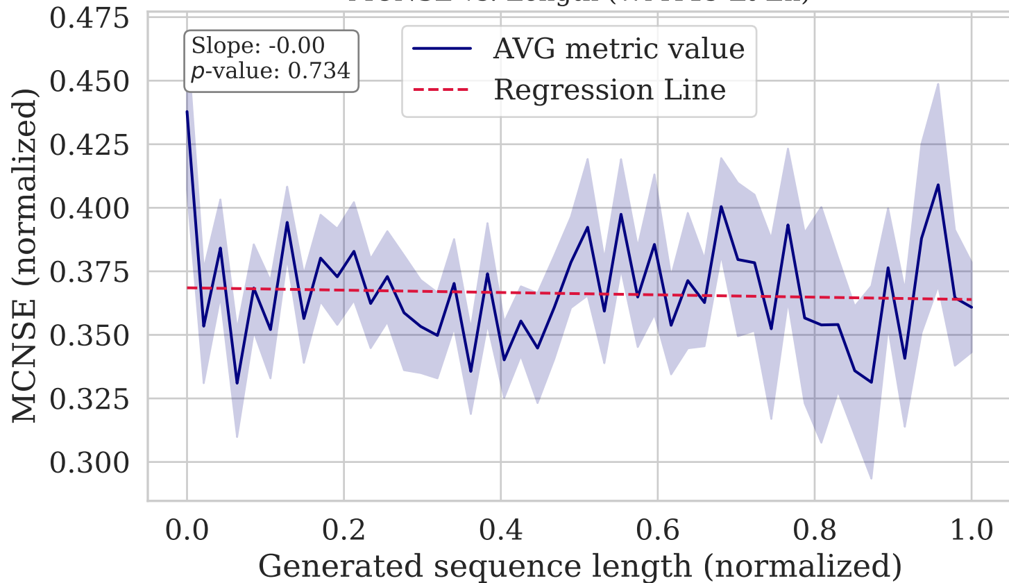
MCNSE vs. Length (WMT19 Lt-En)
