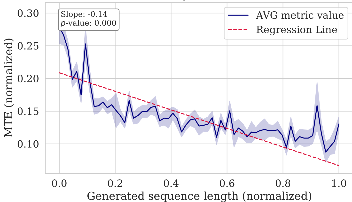
MTE vs. Length (WMT19 Ru-En)
