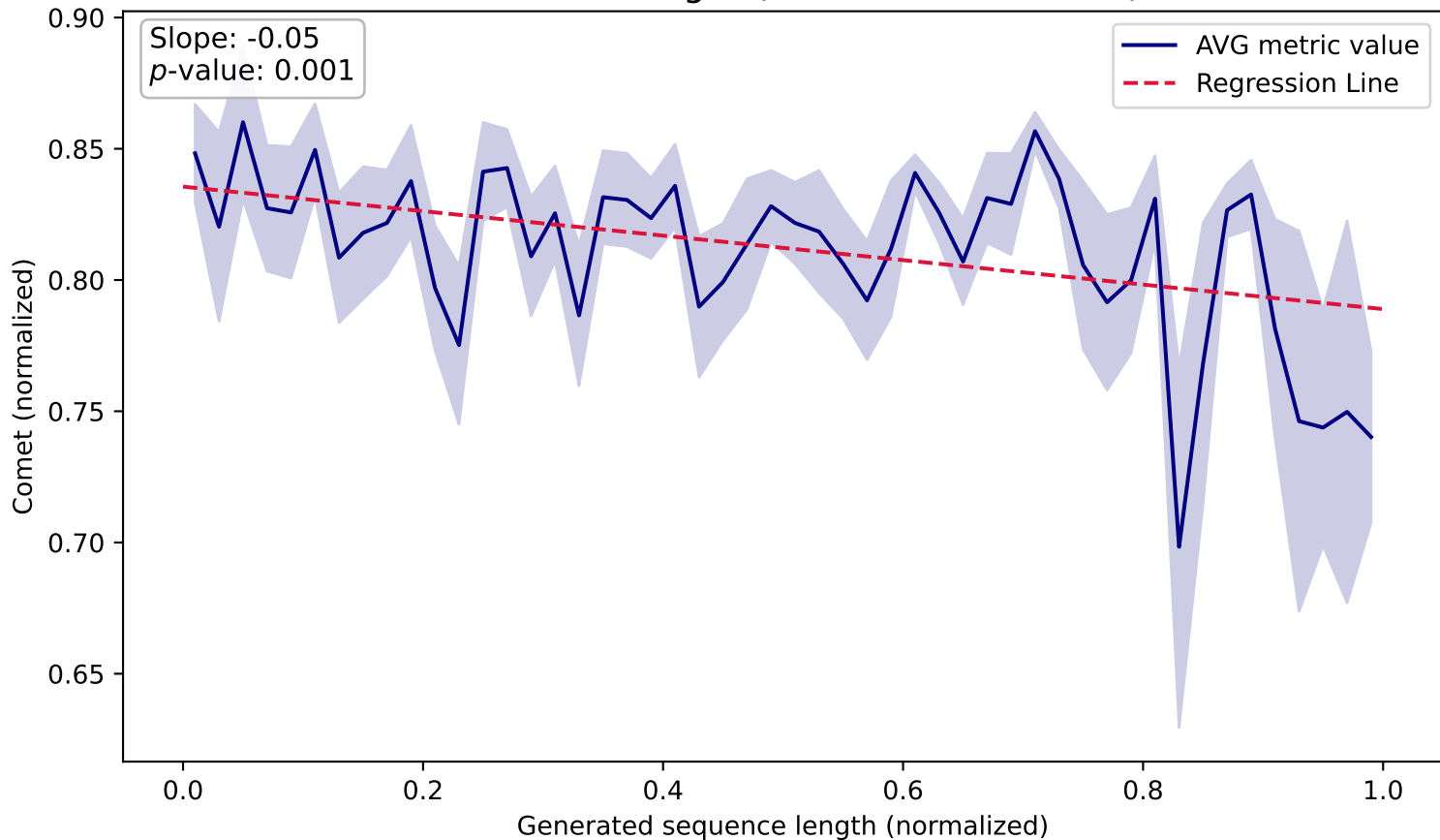
Comet vs. Length (WMT14 Cs-En, Train)
