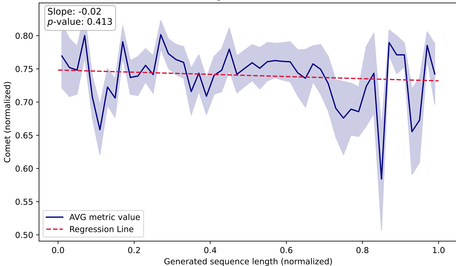
Comet vs. Length (WMT14 De-En, Train)
