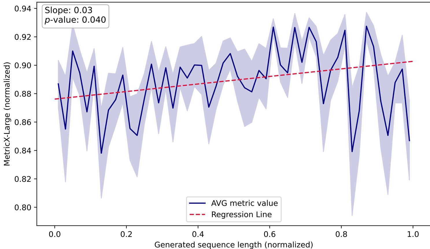
MetricX-Large vs. Length (WMT14 Cs-En, Train)
