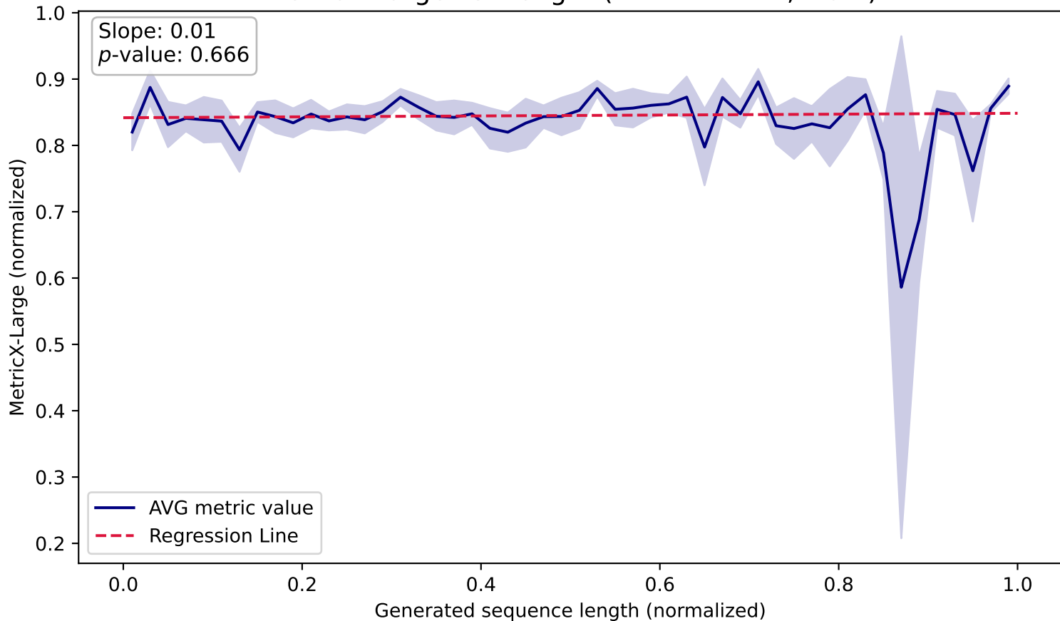
MetricX-Large vs. Length (WMT14 Fr-En, Train)
