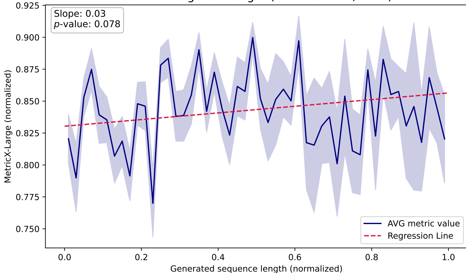
MetricX-Large vs. Length (WMT19 Lt-En, Train)
