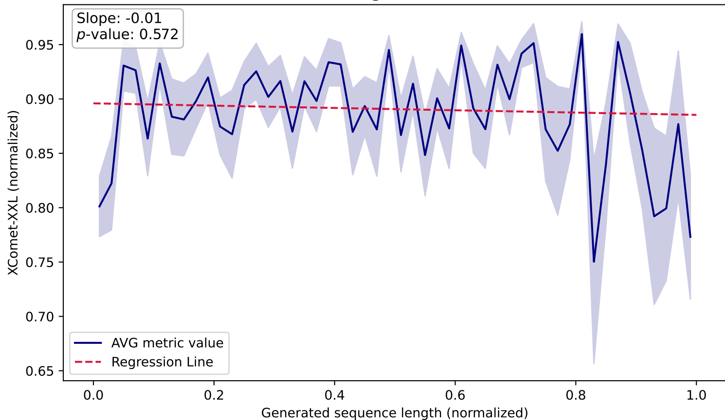
XComet-XXL vs. Length (WMT14 Cs-En, Train)
