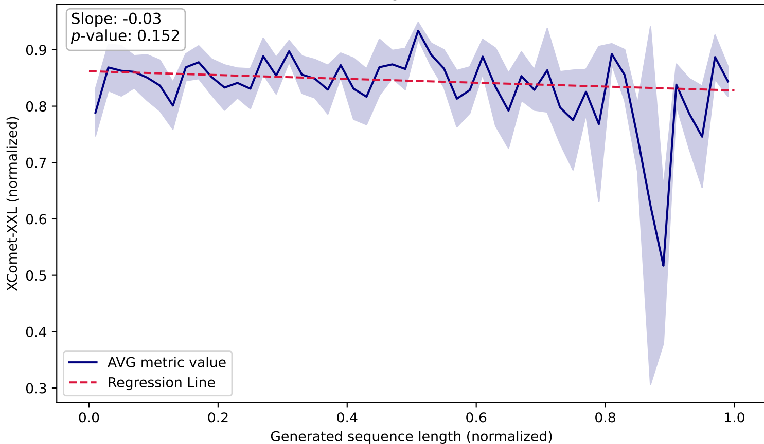
XComet-XXL vs. Length (WMT14 Fr-En, Train)
