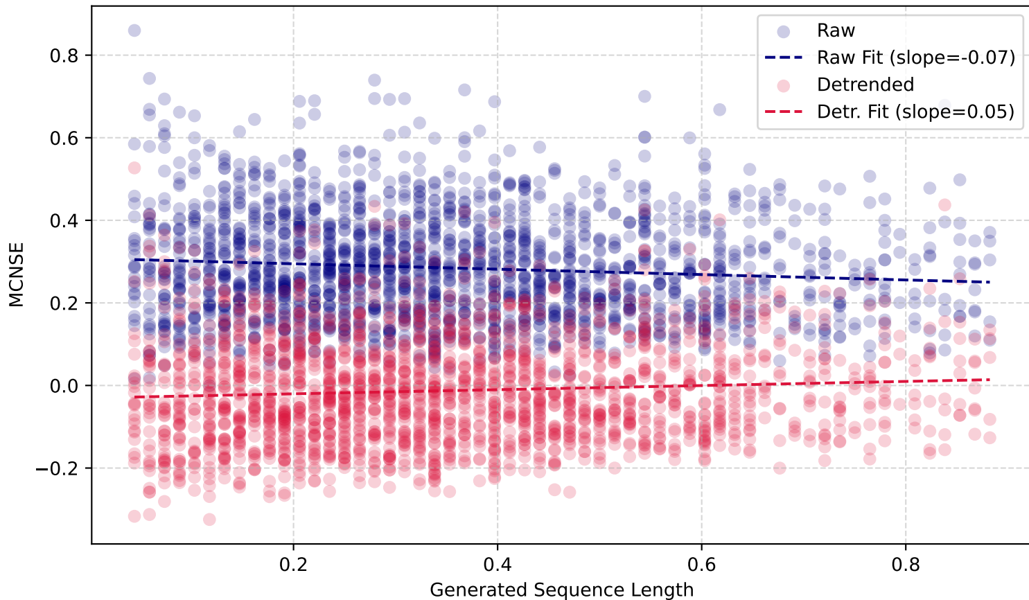
MCNSE vs. Length (WMT19 Ru-En)
