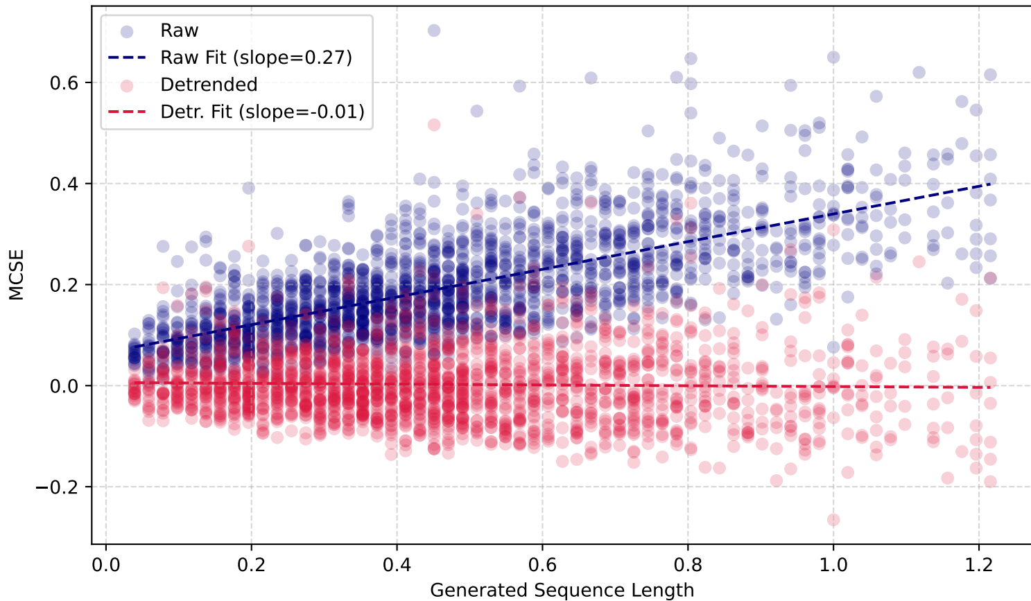
MCSE vs. Length (WMT19 Lt-En)
