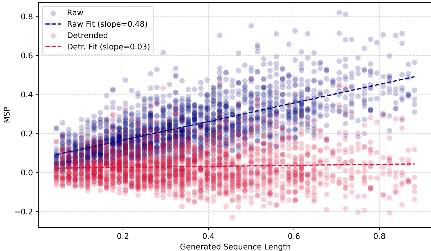
MSP vs. Length (WMT19 Ru-En)
