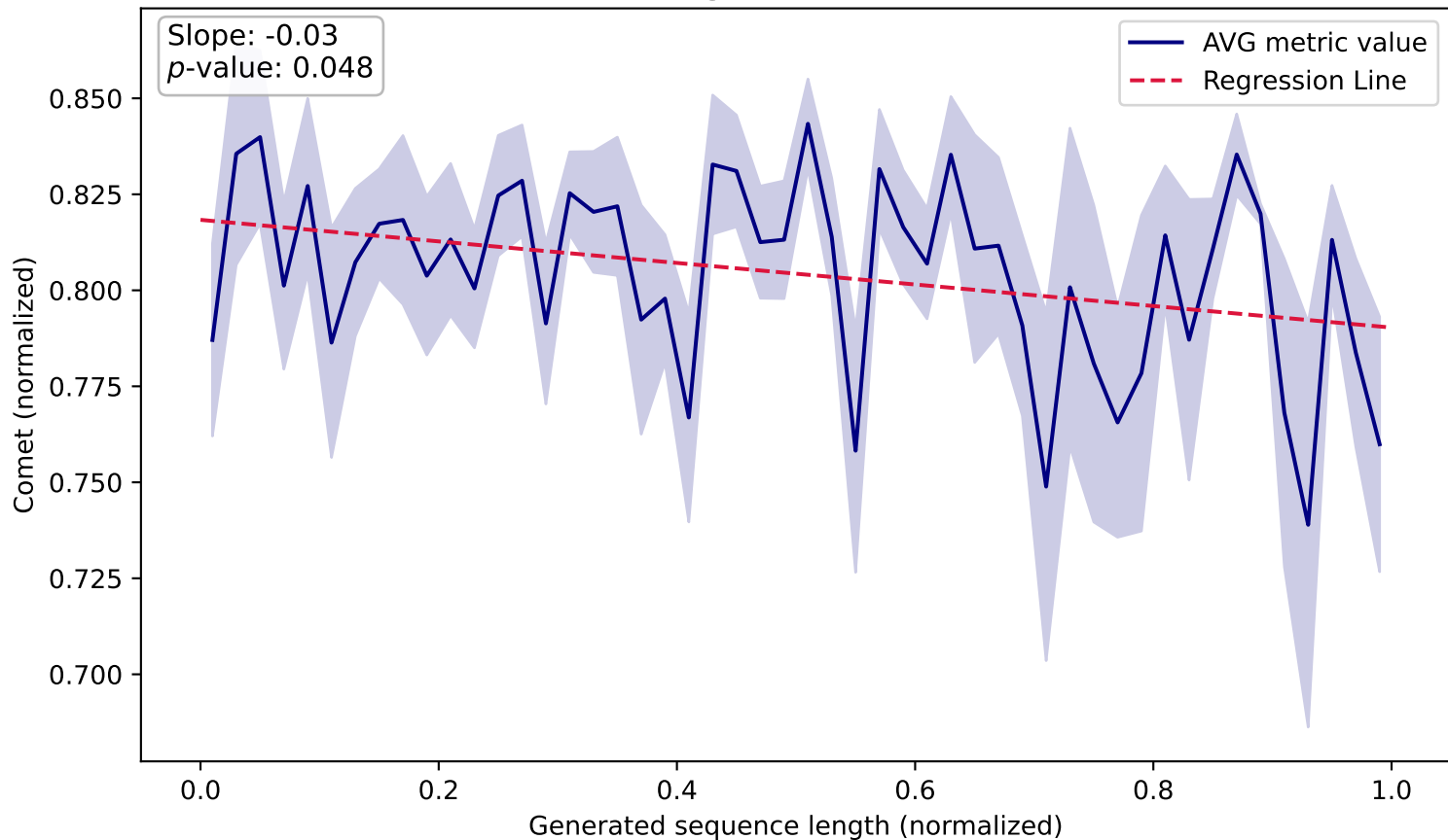
Comet vs. Length (WMT14 Fr-En, Train)
