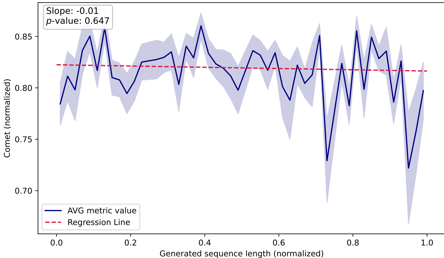
Comet vs. Length (WMT19 Fi-En, Train)
