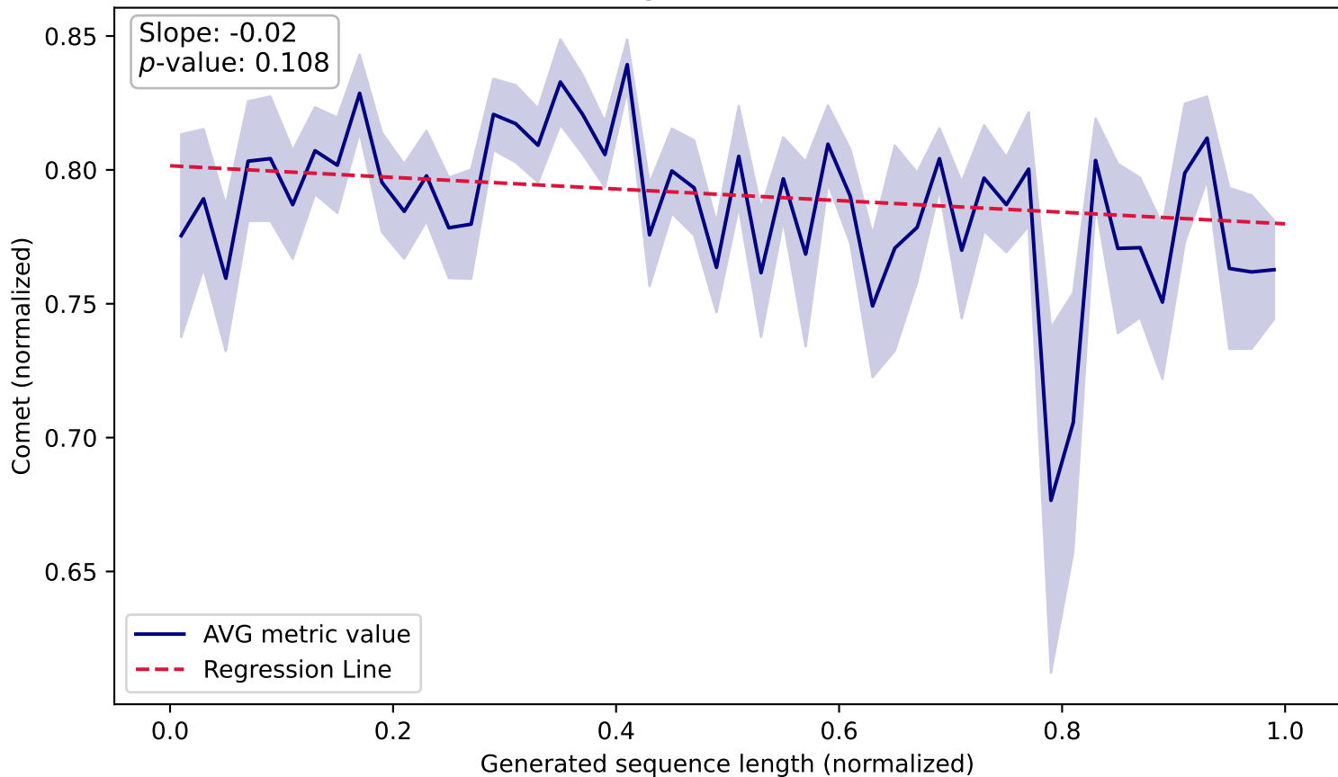
Comet vs. Length (WMT19 Lt-En, Train)
