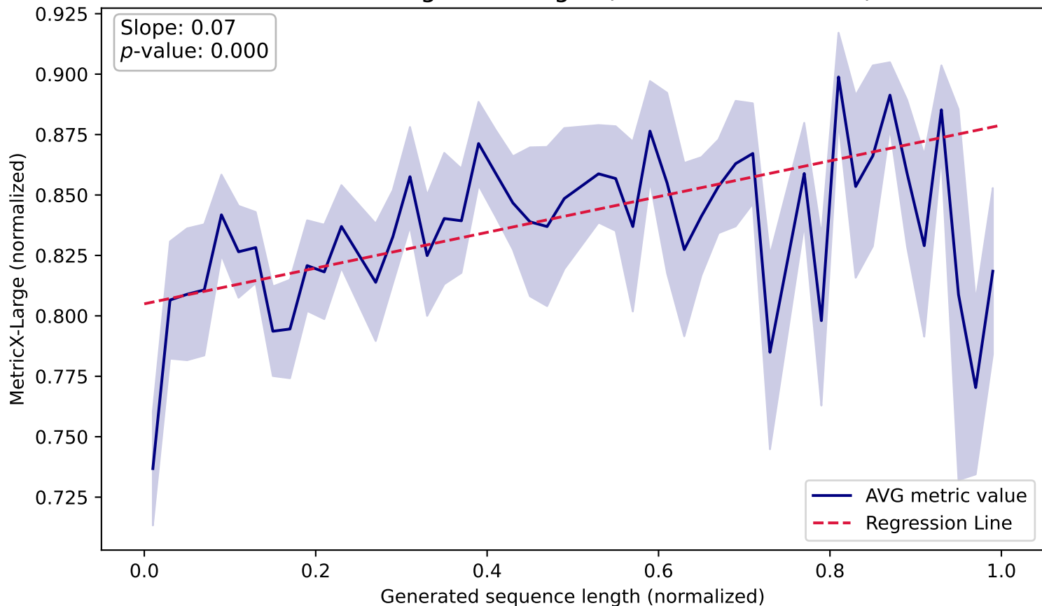
MetricX-Large vs. Length (WMT19 Fi-En, Train)
