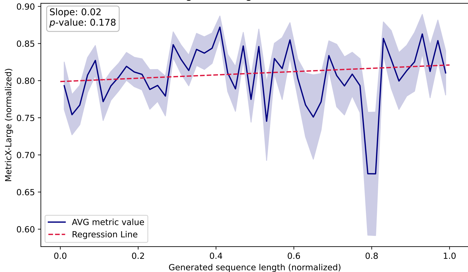
MetricX-Large vs. Length (WMT19 Lt-En, Train)
