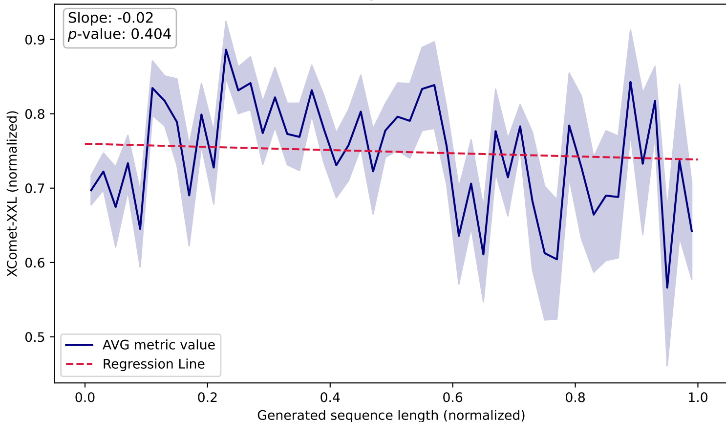
XComet-XXL vs. Length (WMT14 Ru-En, Train)
