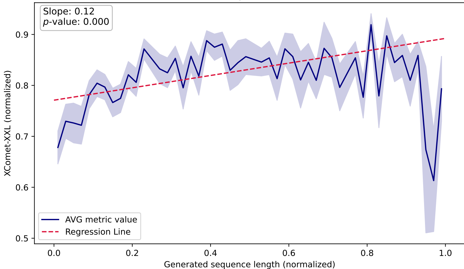
XComet-XXL vs. Length (WMT19 Fi-En, Train)
