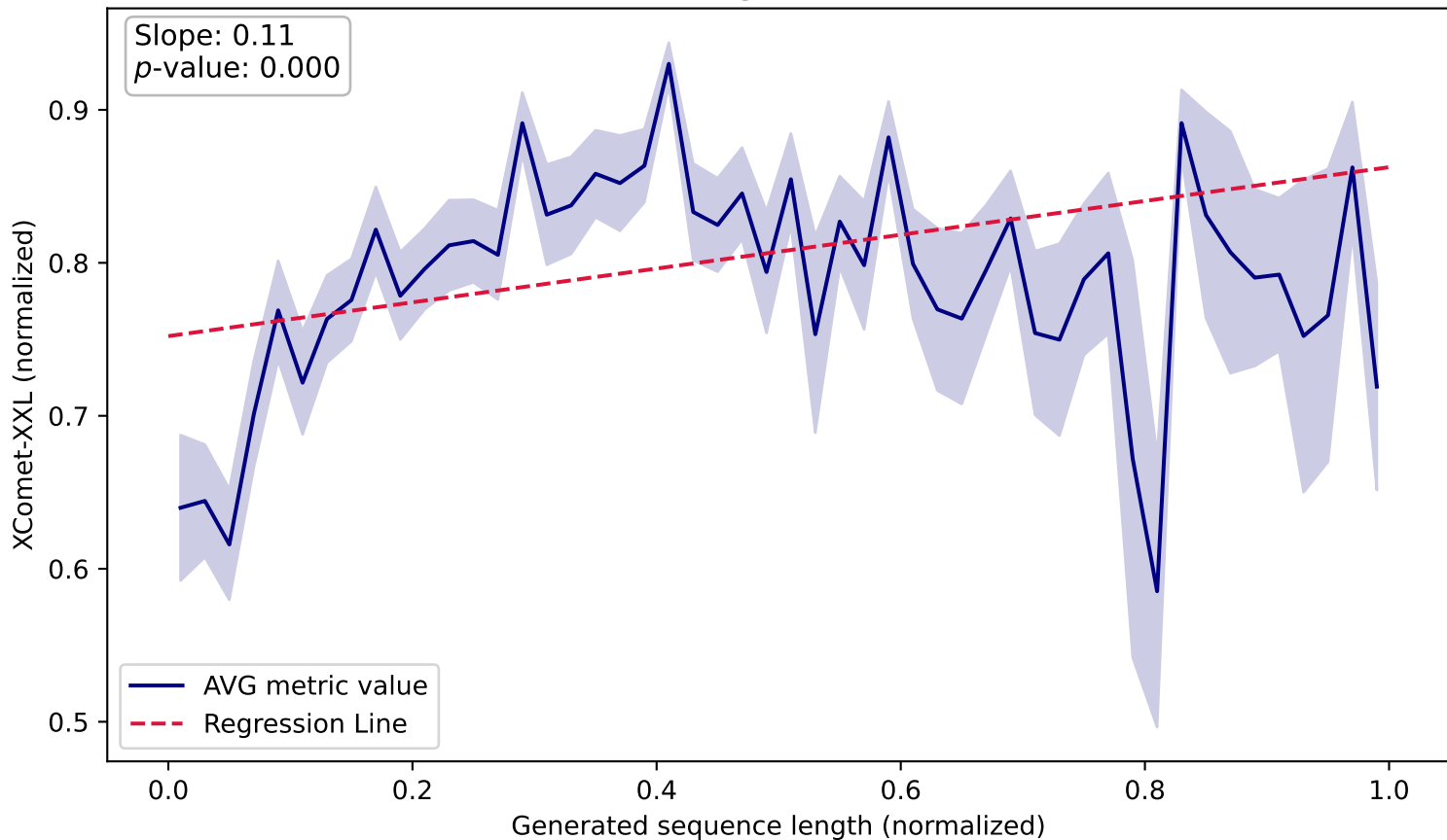
XComet-XXL vs. Length (WMT19 Lt-En, Train)
