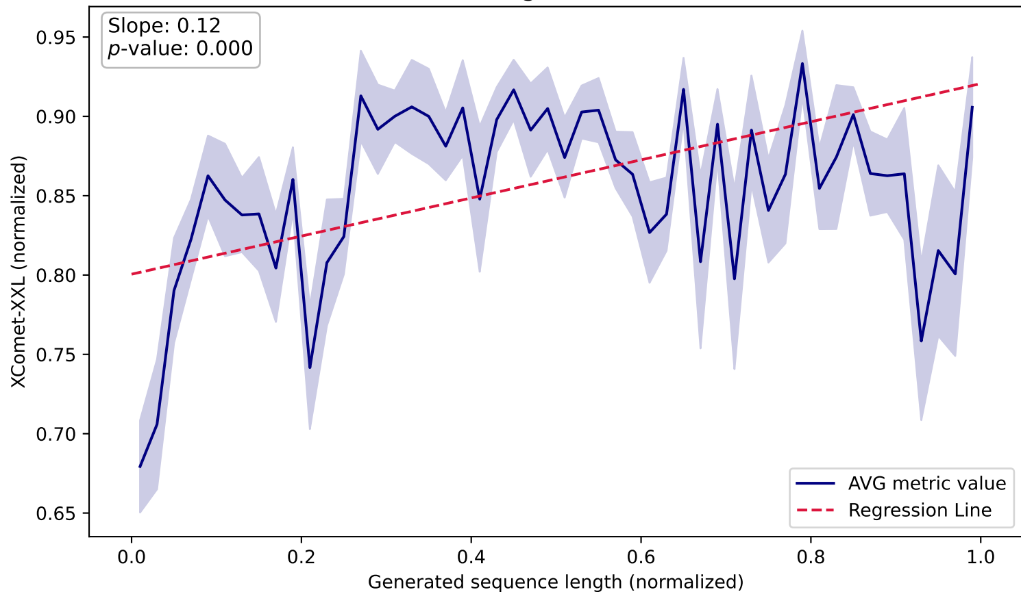
XComet-XXL vs. Length (WMT19 Ru-En, Train)
