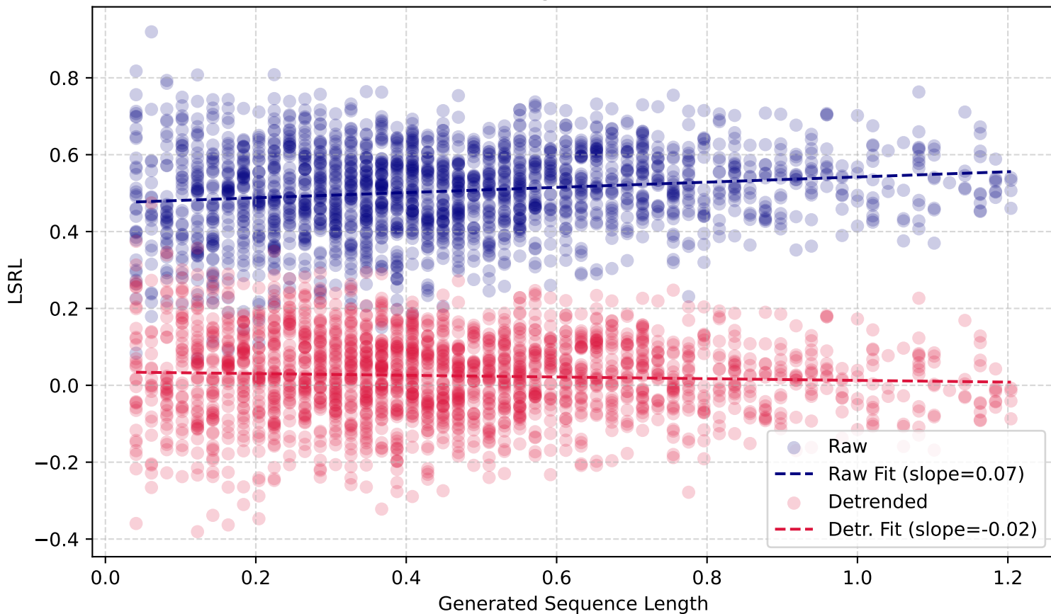
LSRL vs. Length (WMT19 Lt-En)
