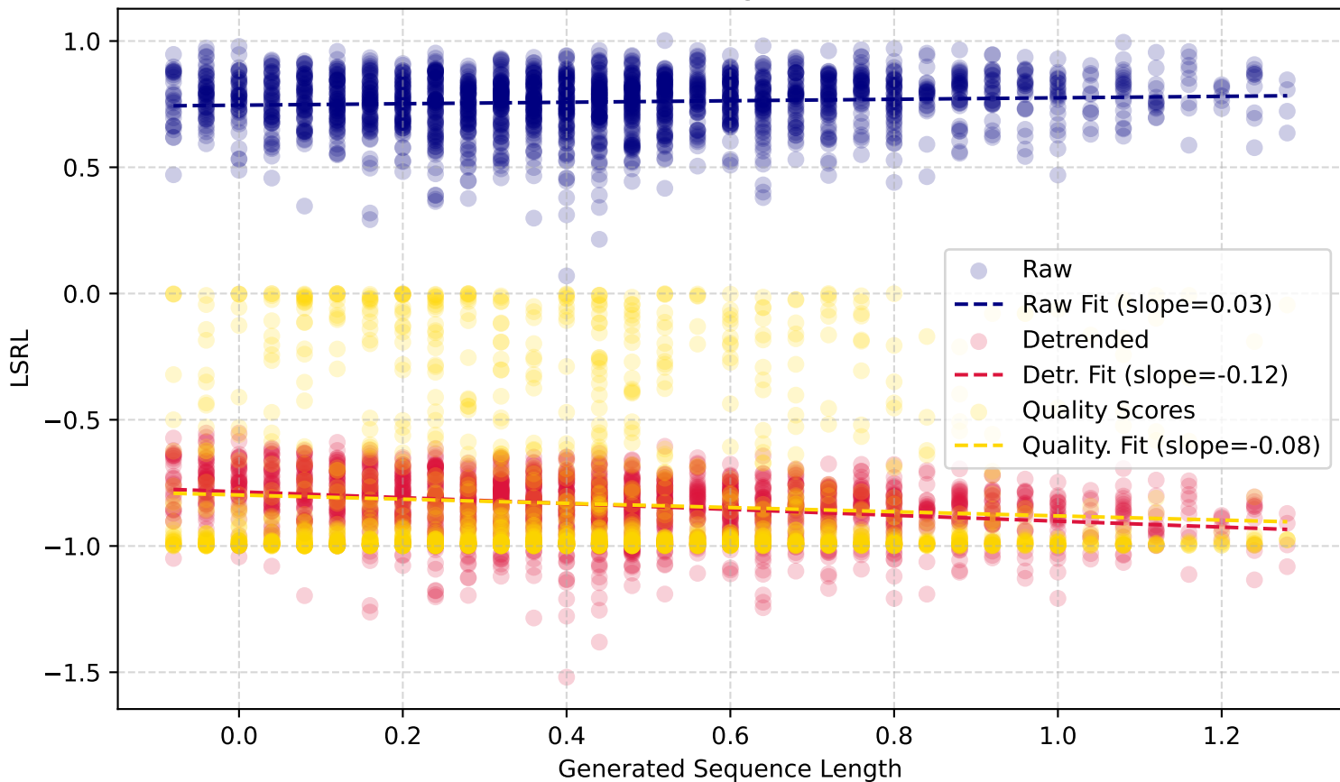
LSRL vs. Length (XSUM)
