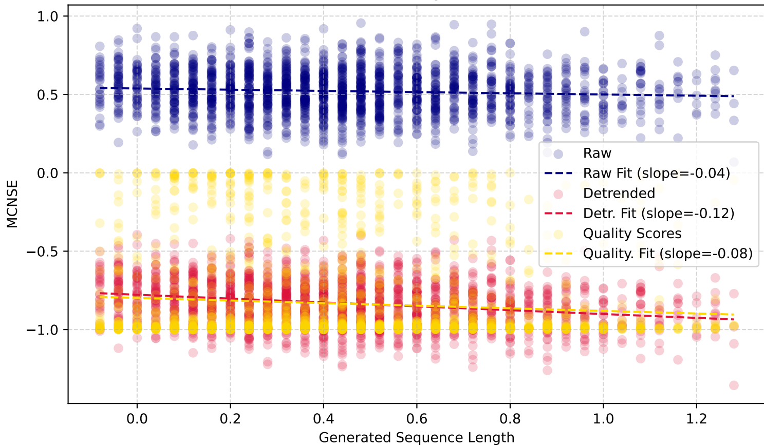
MCNSE vs. Length (XSUM)
