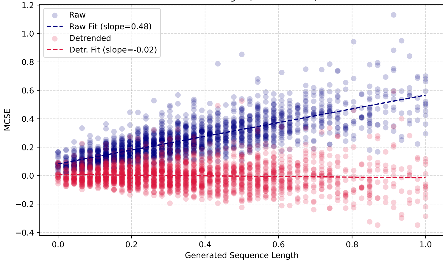
MCSE vs. Length (WMT19 Fi-En)
