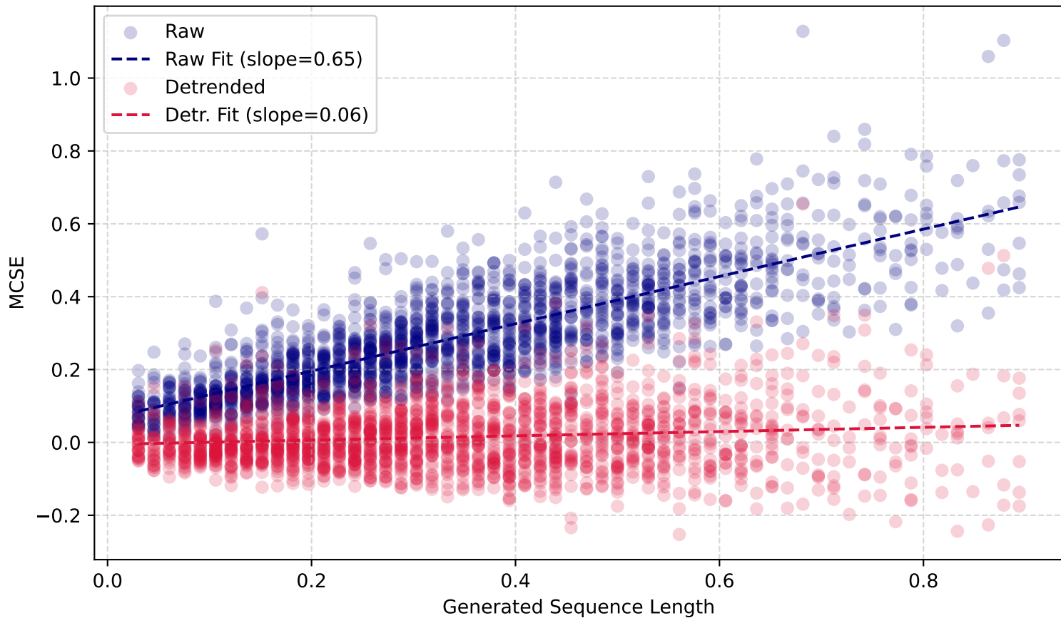
MCSE vs. Length (WMT19 Ru-En)
