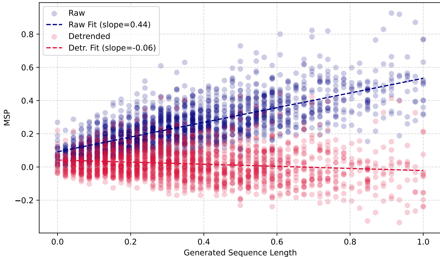
MSP vs. Length (WMT19 Fi-En)
