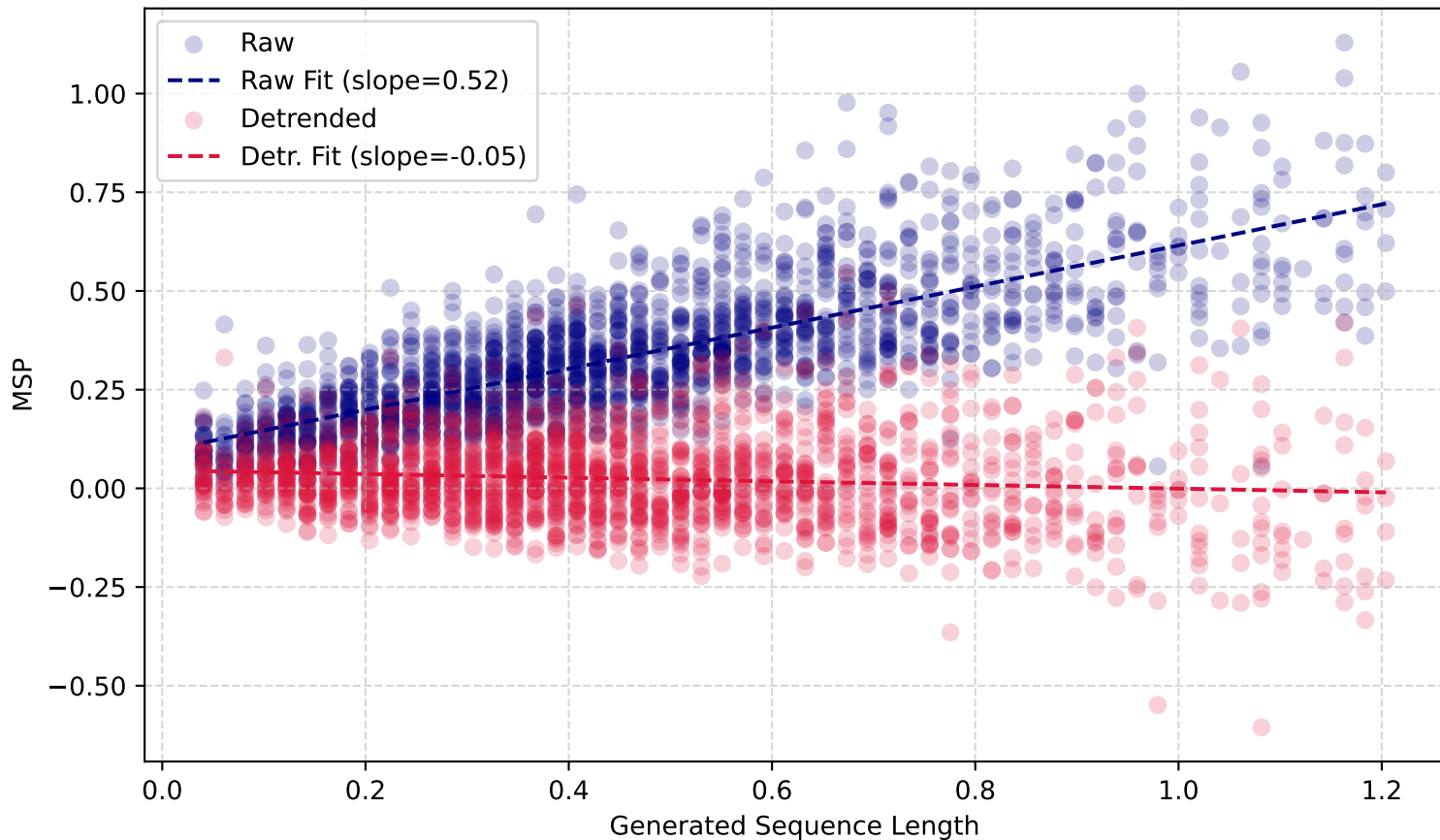
MSP vs. Length (WMT19 Lt-En)
