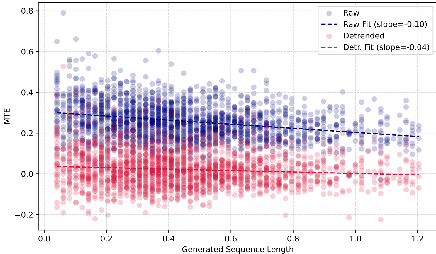
MTE vs. Length (WMT19 Lt-En)
