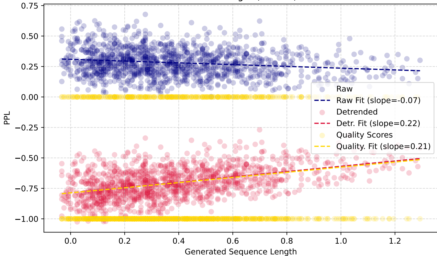
PPL vs. Length (GSM8K)
