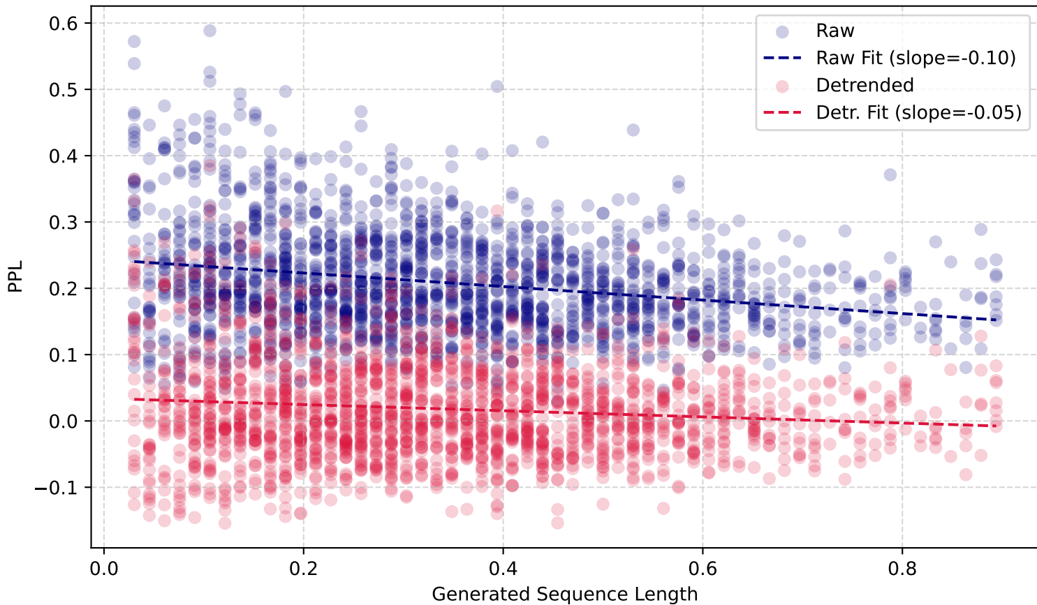
PPL vs. Length (WMT19 Ru-En)
