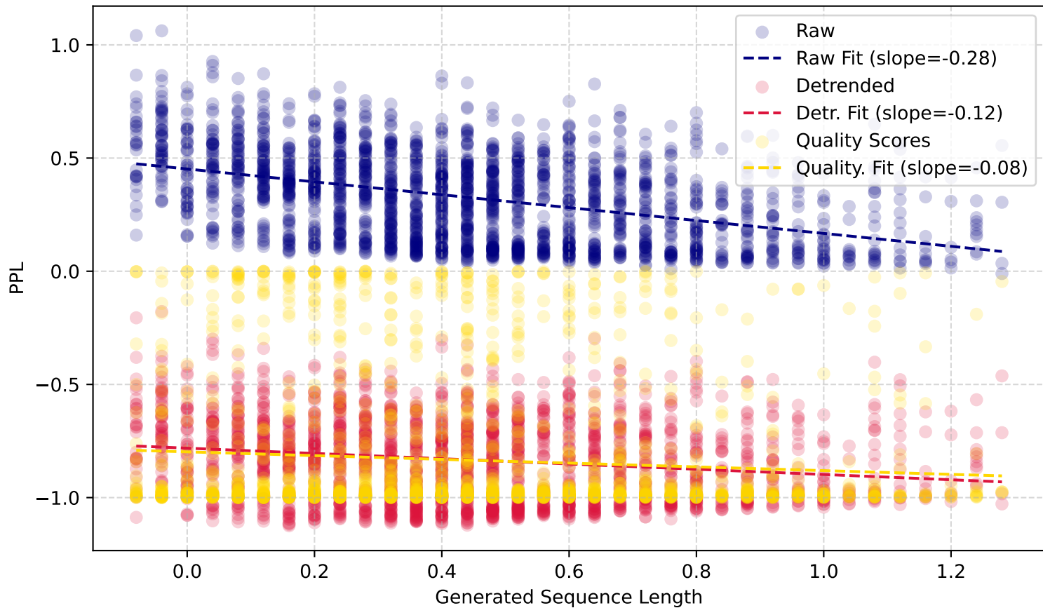
PPL vs. Length (XSUM)
