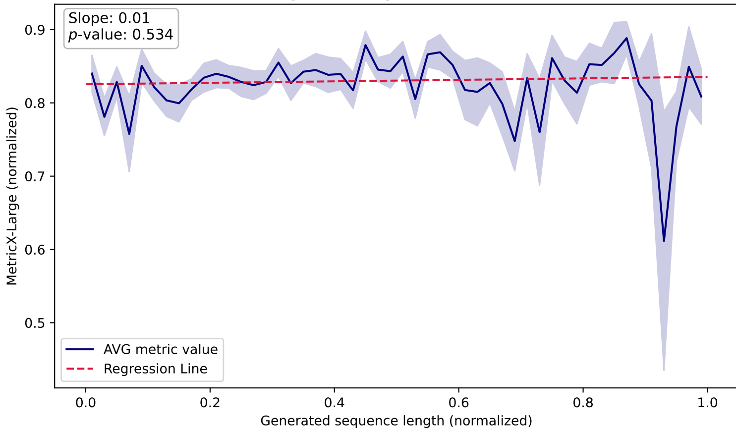
MetricX-Large vs. Length (WMT14 Fr-En, Train)
