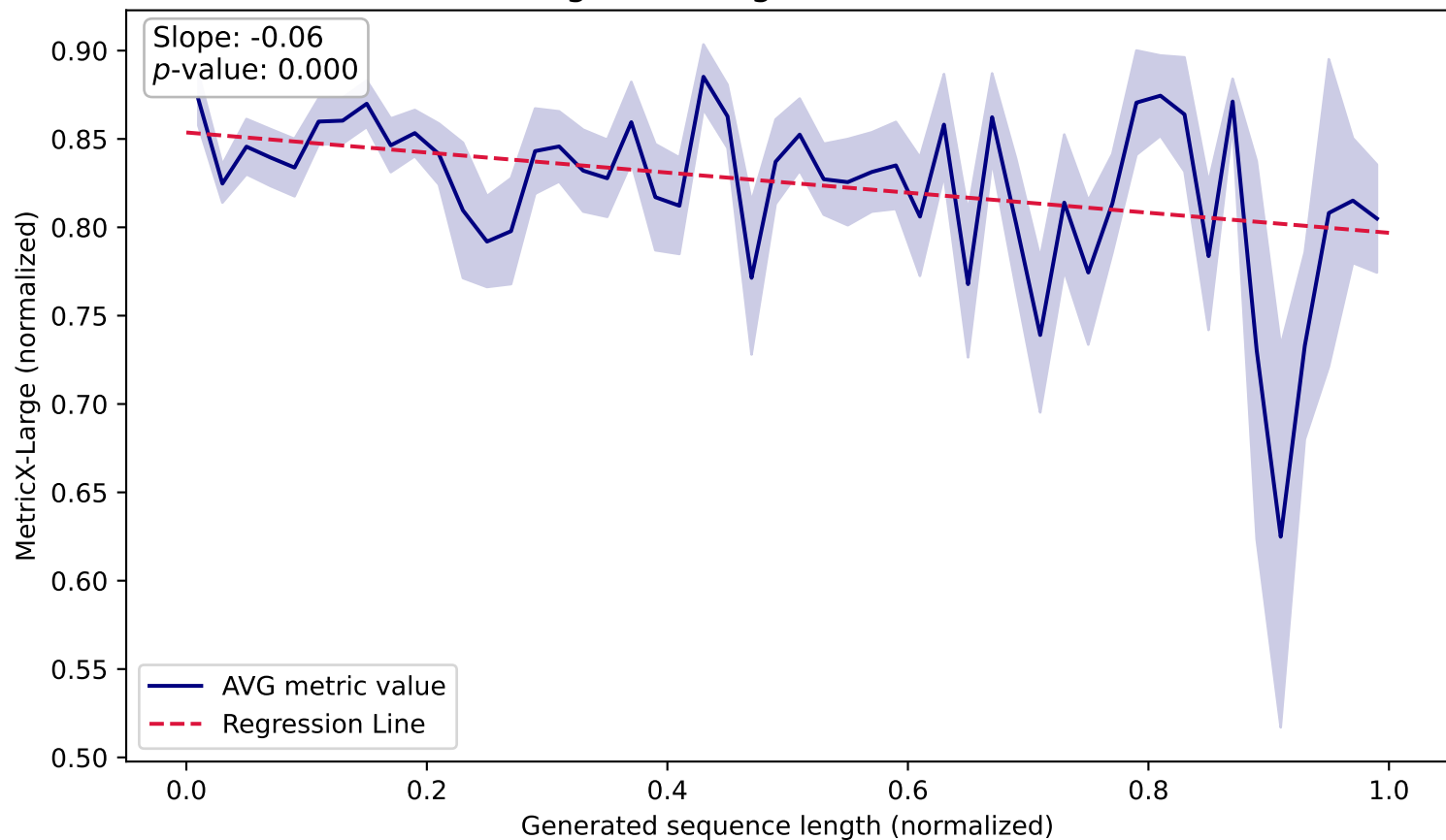
MetricX-Large vs. Length (WMT19 De-En, Train)
