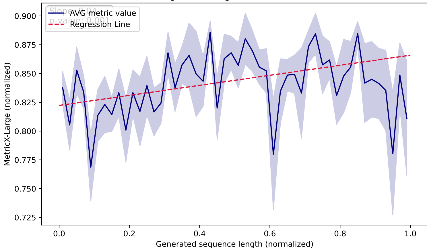
MetricX-Large vs. Length (WMT19 Ru-En, Train)
