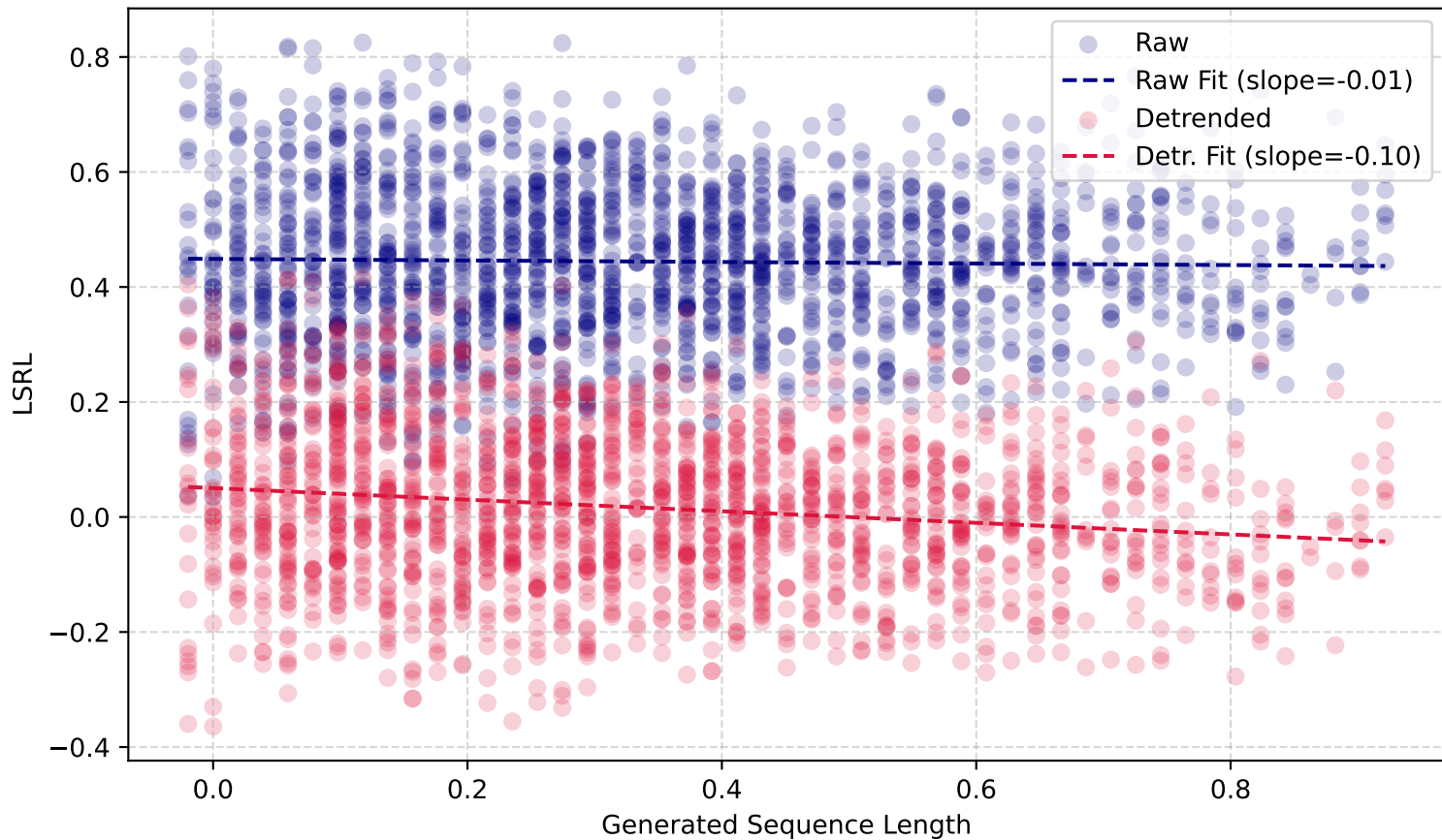
LSRL vs. Length (WMT19 De-En)
