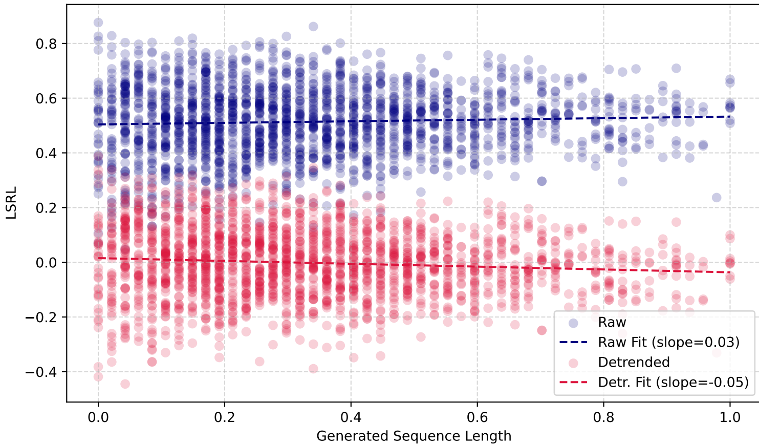
LSRL vs. Length (WMT19 Fi-En)
