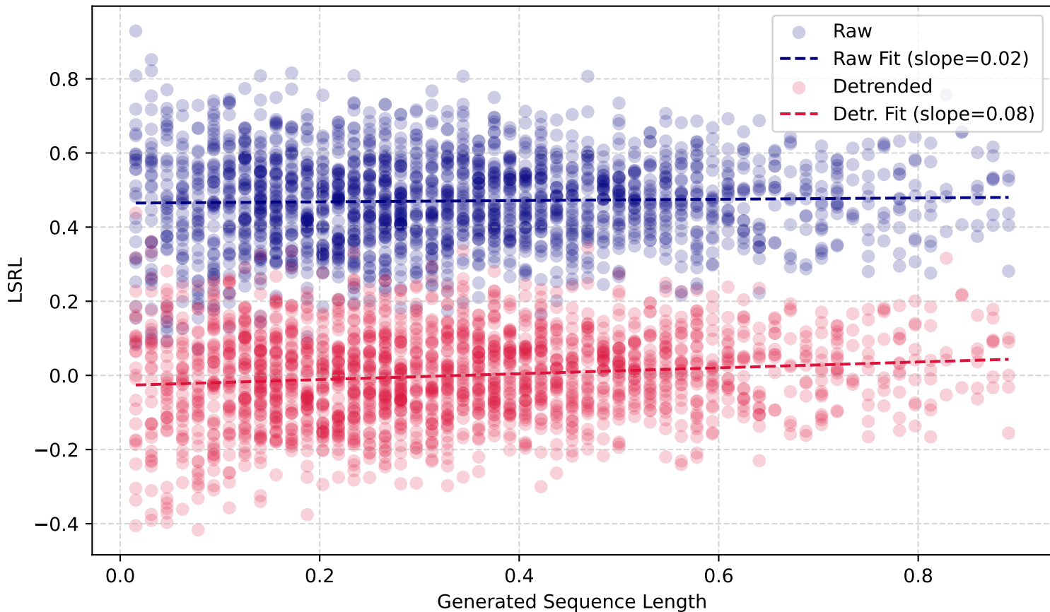
LSRL vs. Length (WMT19 Ru-En)
