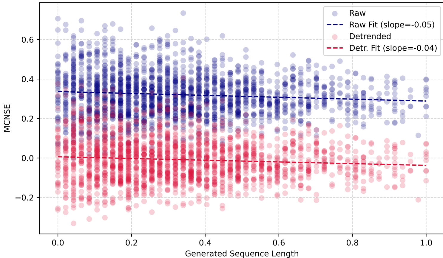
MCNSE vs. Length (WMT19 Fi-En)
