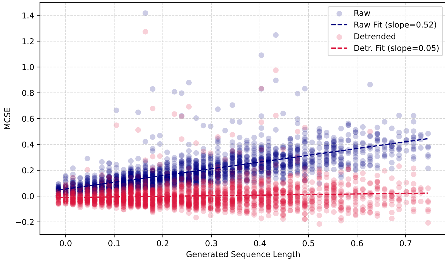
MCSE vs. Length (WMT14 Fr-En)
