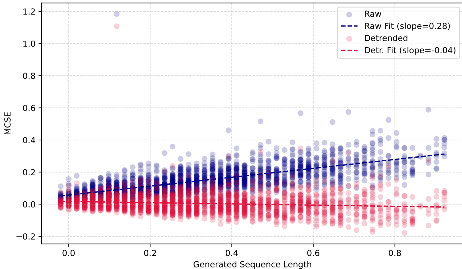
MCSE vs. Length (WMT19 De-En)
