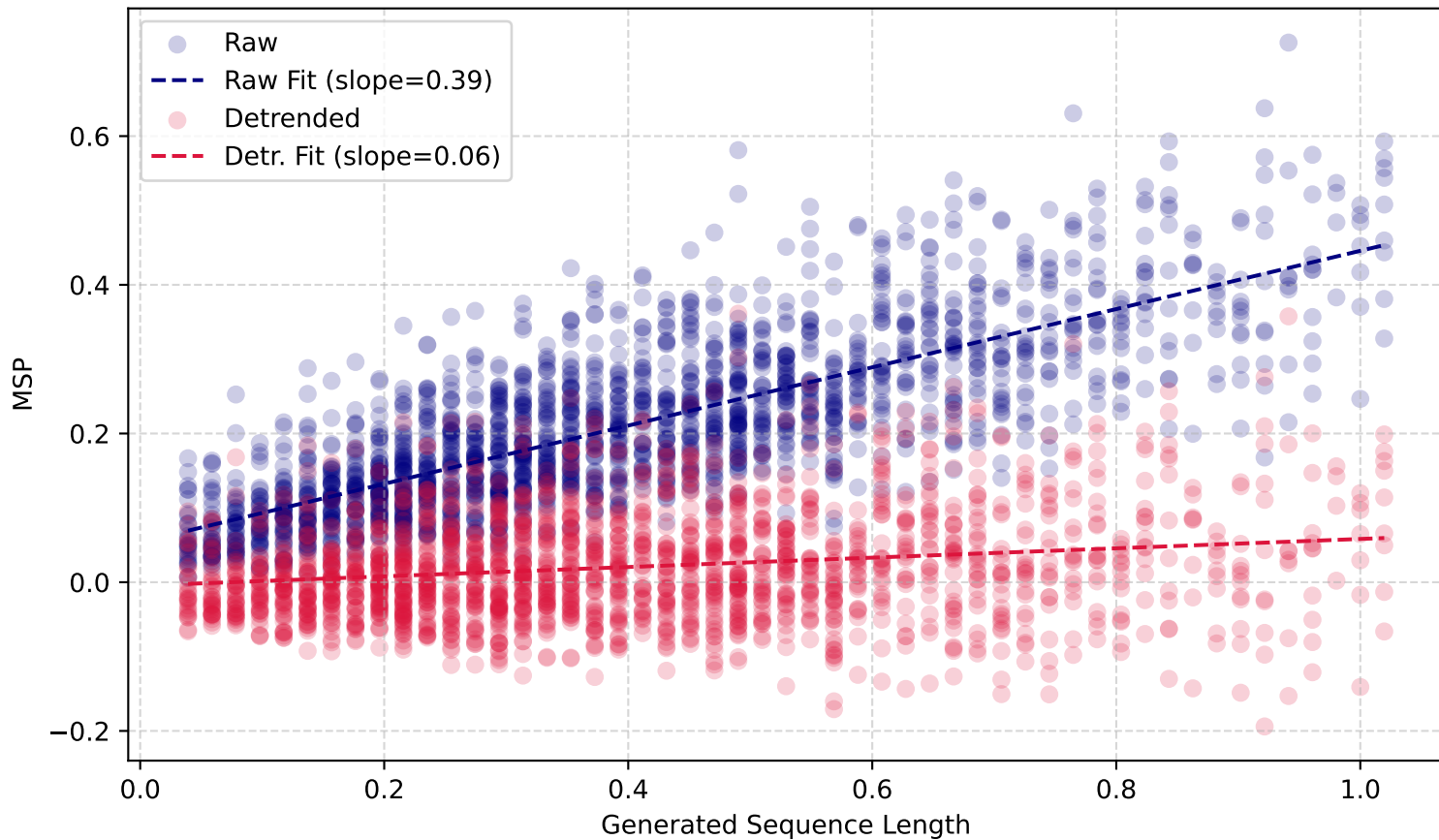
MSP vs. Length (WMT14 Ru-En)
