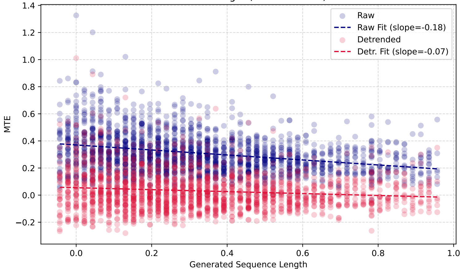
MTE vs. Length (WMT14 De-En)
