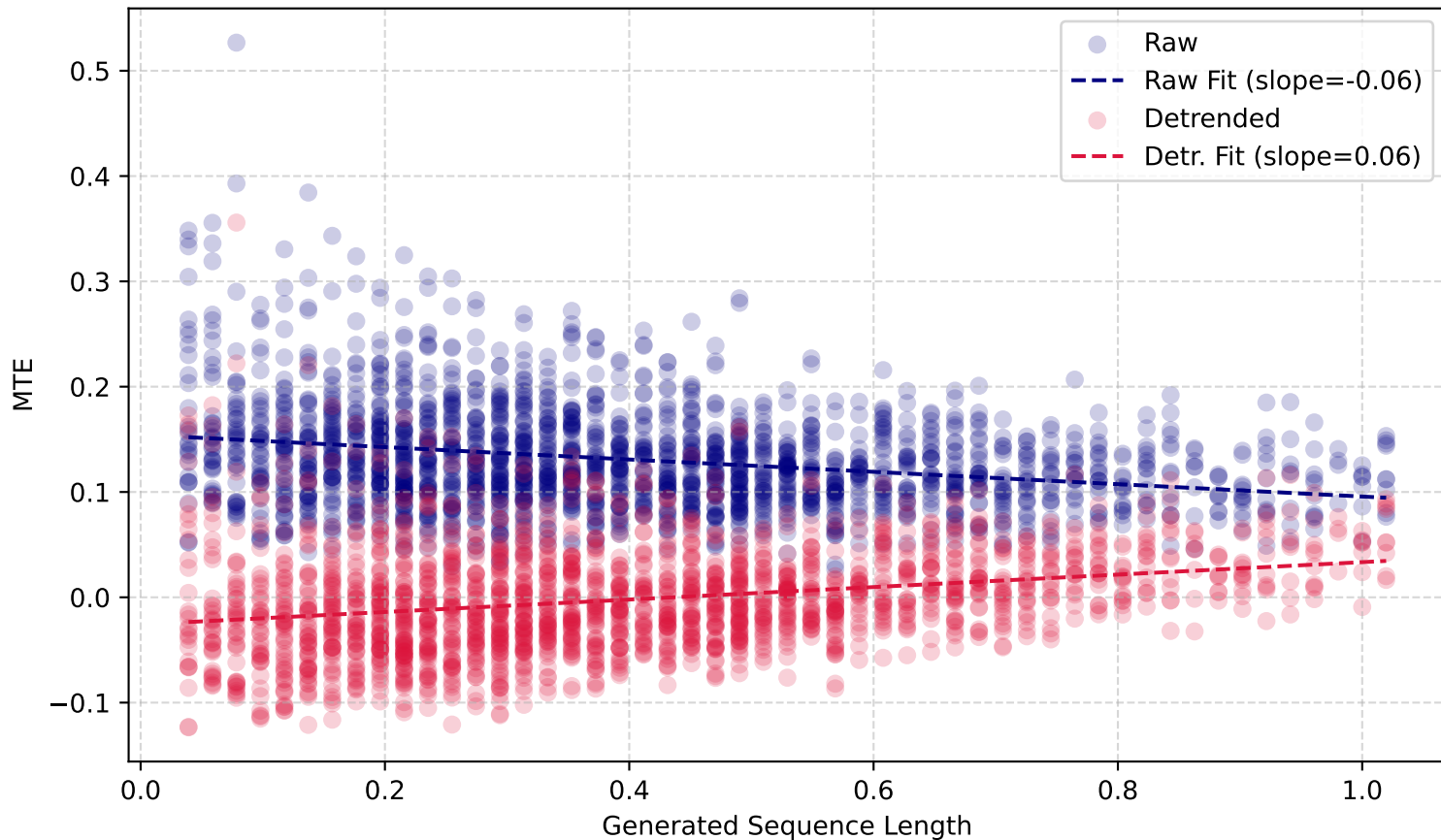
MTE vs. Length (WMT14 Ru-En)
