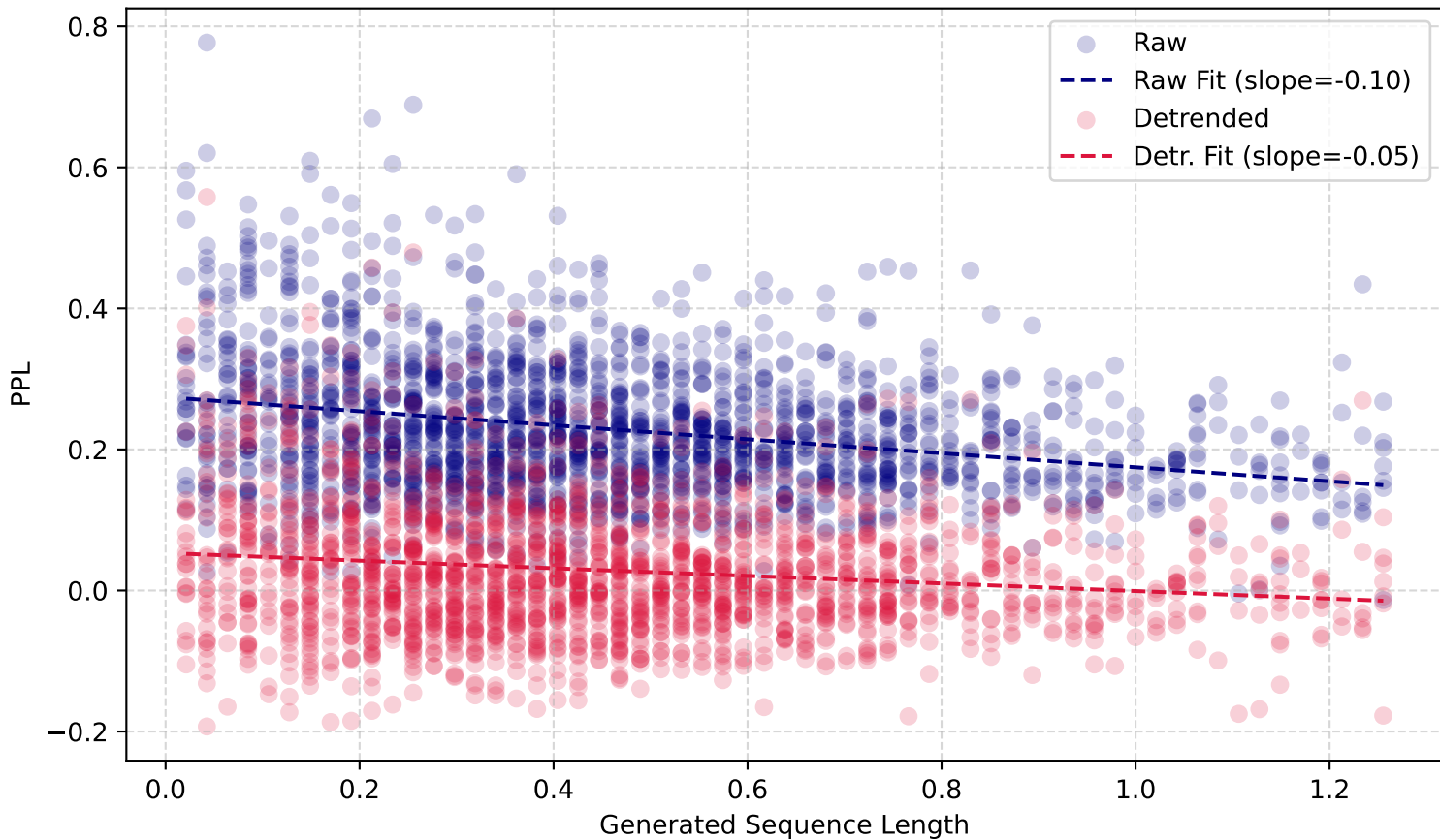
PPL vs. Length (WMT19 Lt-En)
