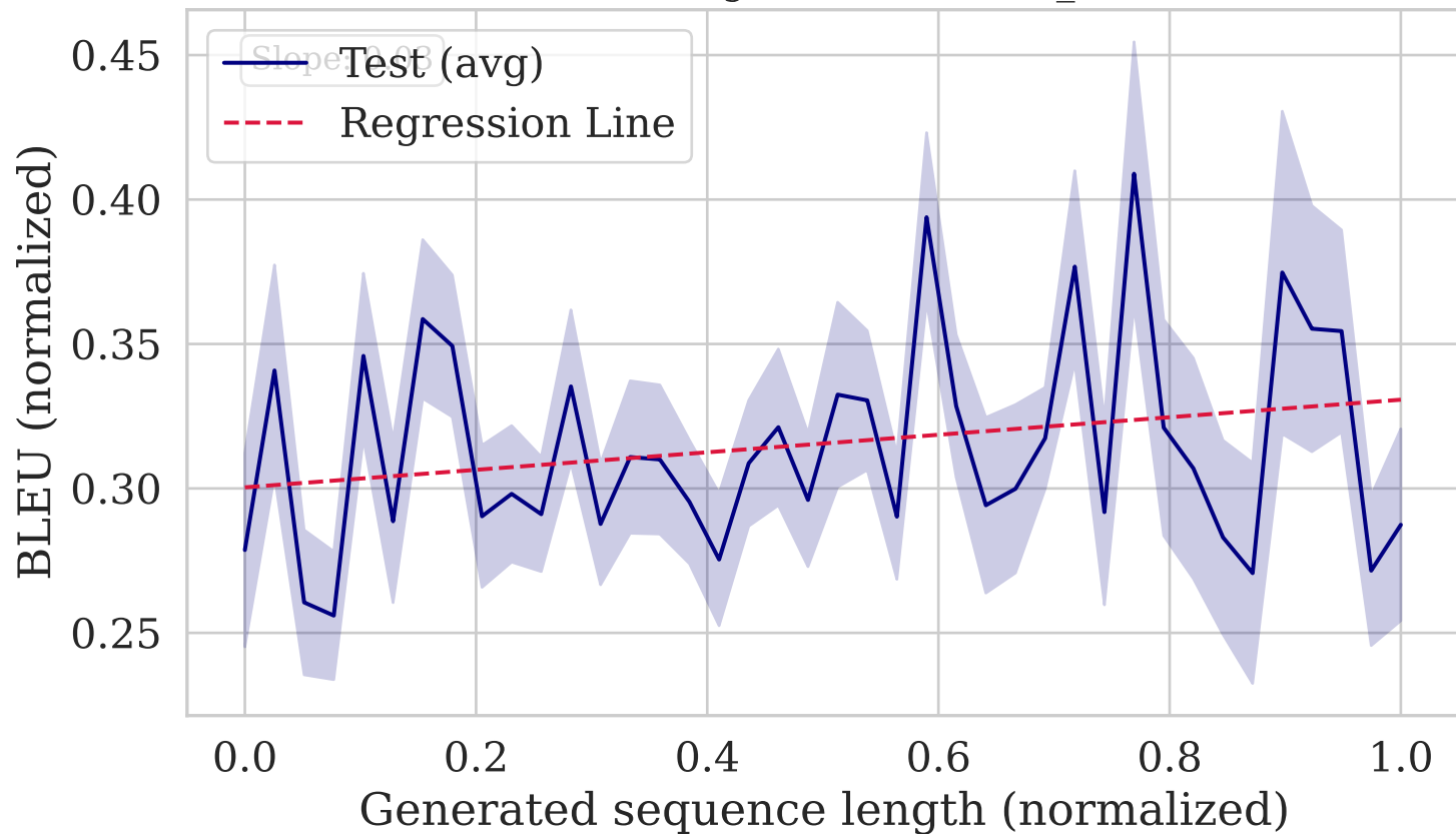
BLEU vs. Length (Test - wmt14_deen)
