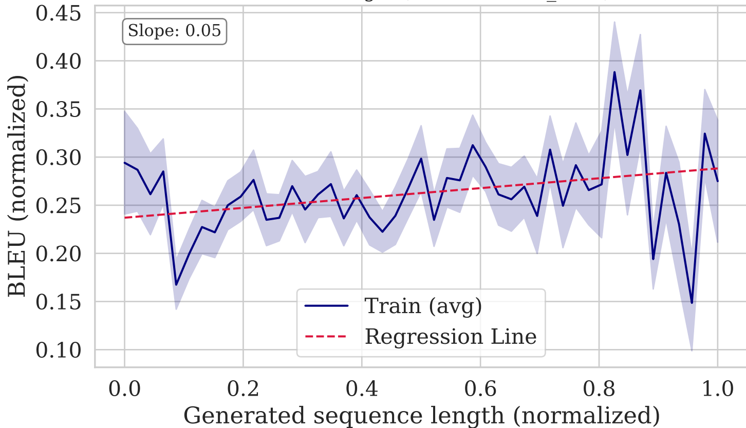
BLEU vs. Length (Train - wmt14_deen)
